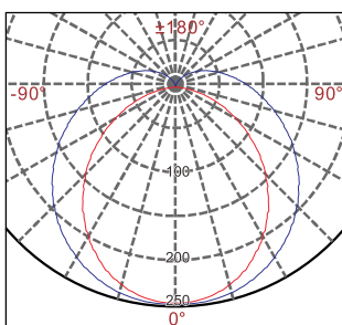
NEVB01 10W 150°
